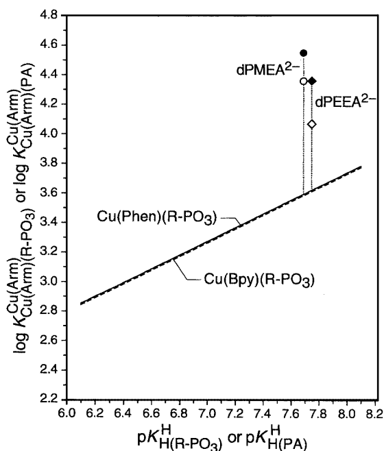
Figure 3. Evidence for an enhanced stability of the ternary \text{Cu}(\text{Bpy})(\text{dPEEA}) ( \diamond ) and \text{Cu}(\text{Phen})(\text{dPEEA}) ( \blacklozenge ) as well as the \text{Cu}(\text{Bpy})(\text{dPMEA}) ( \circ ) and \text{Cu}(\text{Phen})(\text{dPMEA}) ( \bullet ) complexes, based on the relationship between \log K_{\text{Cu}(\text{Arm})/\text{Cu}(\text{Arm})(\text{R-PO}_3)} or \log K_{\text{Cu}(\text{Arm})/\text{Cu}(\text{Arm})(\text{PA})} and \text{pK}_{\text{H}}^{\text{H}}(\text{R-PO}_3) or \text{pK}_{\text{H}}^{\text{H}}(\text{PA}) in aqueous solution at I = 0.1 \text{ M} ( \text{NaNO}_3 ) and 25^\circ\text{C} . The plotted data corresponding to the \text{dPEEA}^{2-} systems are from Tables 1 and 5 and those corresponding to \text{dPMEA}^{2-} are from ref. [38] The two reference lines represent the \log K versus \text{pK}_{\text{a}} relationship for the ternary \text{Cu}(\text{Arm})(\text{R-PO}_3) complexes [Equation (10)]; it should be emphasized that \text{R-PO}_3^{2-} symbolizes here phosph(on)ate ligands with a group R unable to undergo any kind of hydrophobic, stacking or other type of interaction. The parameters for the straight-line equations are listed in ref. [61]
