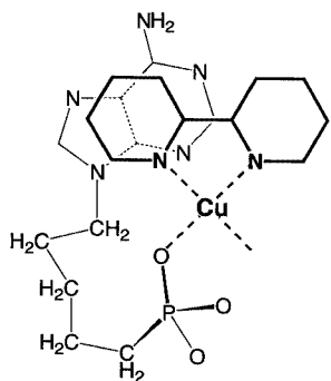
Figure 4. Tentative and simplified structure of a species with an intramolecular stack for Cu(Bpy)(dPMEA) in solution. The orientation of the aromatic rings may vary somewhat from one stacked species to the next; such a stacked complex in solution should not be considered as being rigid.
