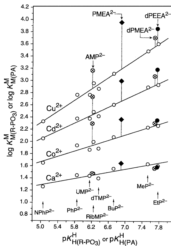
Figure 2. Evidence for an enhanced stability of the \text{Cd(dPEEA)} and \text{Cu(dPEEA)} and possibly also the \text{Co(dPEEA)} complexes, and for the lack of such an enhanced stability of the \text{Ca(dPEEA)} species (●), together with the data points for the corresponding metal ion complexes of \text{dPMEA}^{2-} , \text{AMP}^{2-} (⊗) and \text{PMEA}^{2-} (◆) based on the relationship between \log K_{\text{M(R-PO}_3\text{)}}^{\text{M}} and \text{p}K_{\text{H(R-PO}_3\text{)}}^{\text{H}} for \text{M(R-PO}_3\text{)} complexes of some simple phosphate monoester and phosphonate ligands ( \text{R-PO}_3^{2-} ) (○): 4-nitrophenyl phosphate ( \text{NPhP}^{2-} ), phenyl phosphate ( \text{PhP}^{2-} ), uridine 5'-monophosphate ( \text{UMP}^{2-} ), D-ribose 5-monophosphate ( \text{RibMP}^{2-} ), thymidine [ = 1-(2\text{-deoxy-}\beta\text{-D-ribofuranosyl)thymine}] 5'\text{-monophosphate (dTMP}^{2-}) , n -butyl phosphate ( \text{BuP}^{2-} ), methanephosphonate ( \text{MeP}^{2-} ), and ethanephosphonate ( \text{EtP}^{2-} ) (from left to right). The least-squares lines [Equation (10)] are drawn through the corresponding 8 data sets (○) taken from [58] for the phosphate monoesters and from [45] for the phosphonates. The points due to the equilibrium constants for the \text{M}^{2+}/\text{dPEEA} systems (●) are based on the values listed in Tables 1 and 2; those for the \text{M}^{2+}/\text{dPMEA} (⊗), \text{M}^{2+}/\text{AMP} (⊗), and \text{M}^{2+}/\text{PMEA} systems (◆) are from [18,23] and [45], respectively. The vertical broken lines emphasize the stability differences from the reference lines; they equal \log \Delta_{\text{M/PA}} as defined in Equation (11). All the plotted equilibrium constants refer to aqueous solutions at 25 °C and I = 0.1 \text{ M} ( \text{NaNO}_3 ).
